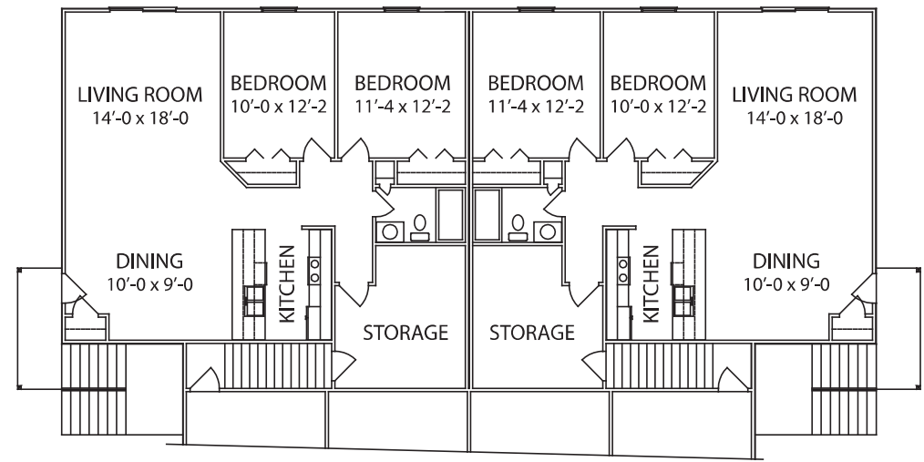
UPPER FLOOR
